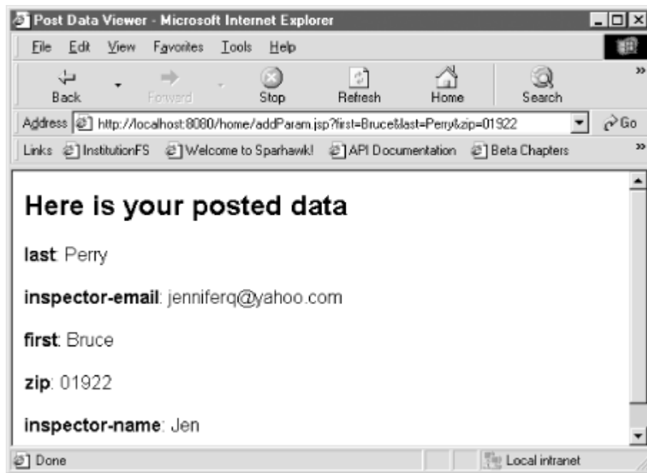
Figure 7-5. Displaying parameters added from a forwarding JSP
