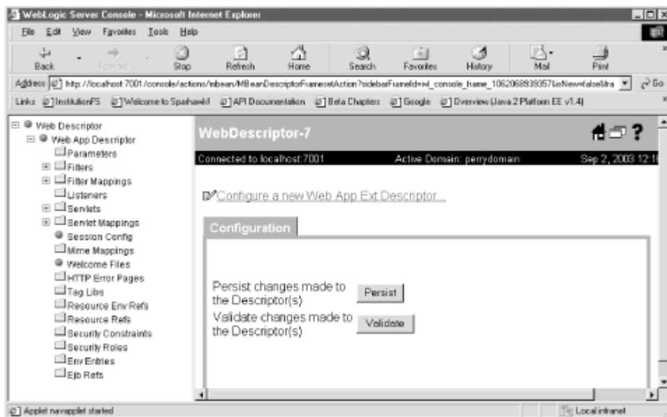
Figure 2-2. Editing the web.xml file graphically
