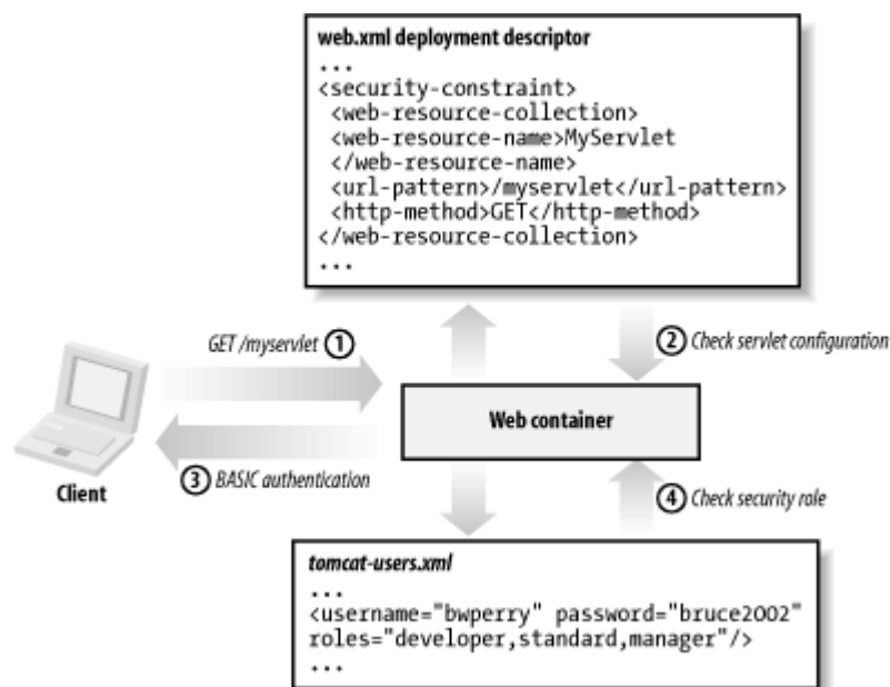
Figure 3-1. Using a security constraint element
