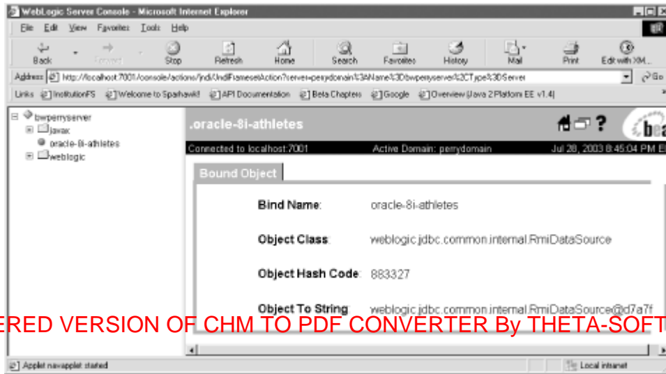
Figure 21-4. A view of the WebLogic JNDI tree containing the DataSource
