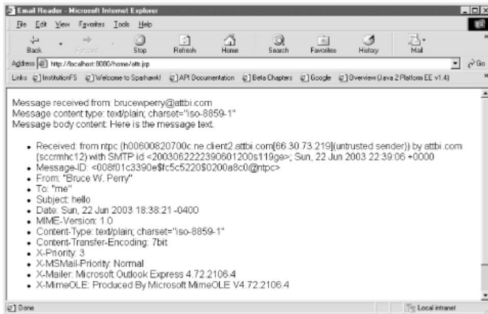
Figure 20-3. A servlet accesses an email and displays its header s
