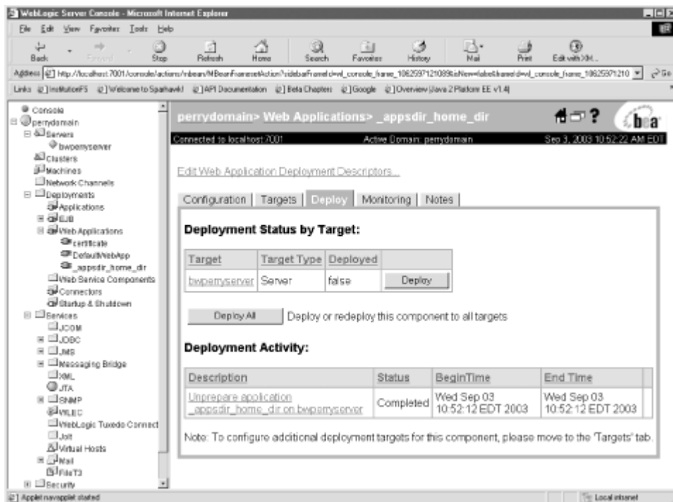
Figure 2-4. Graphically deploying a servlet
