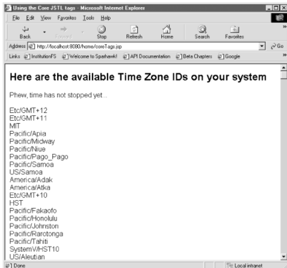
Figure 23-1. A JSP using the various core tags to display time zone I
