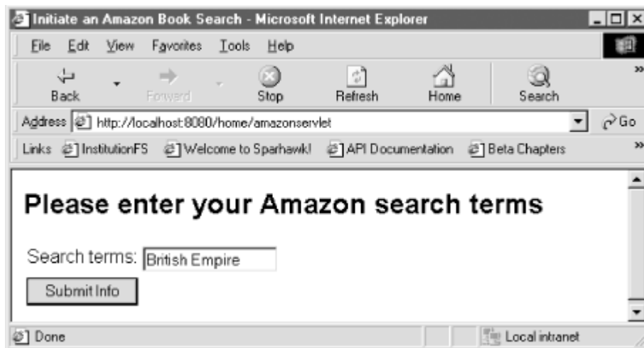
Figure 27-3. A servlet's HTML form accepts Amazon search terms
