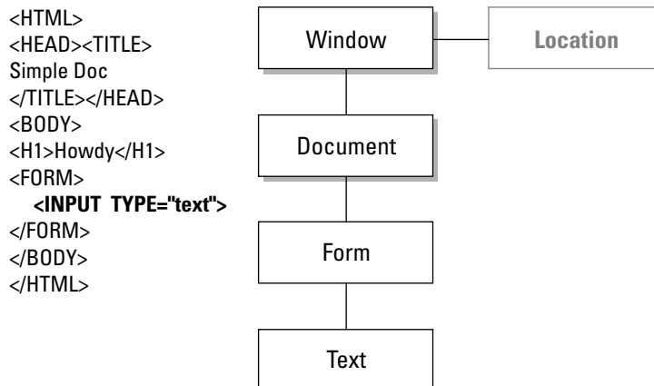
Figure 4-9: Adding a text input element to the form
