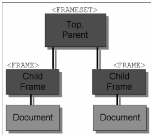
Figure 11-2: Two-frame window and document hierarchy
