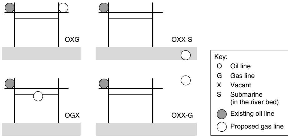
Figure 23.6—River-crossing options
