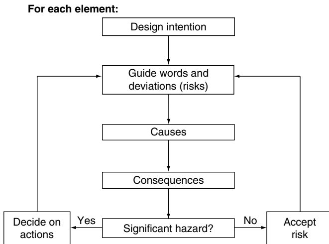
Figure 17.3 —The Hazop study process
