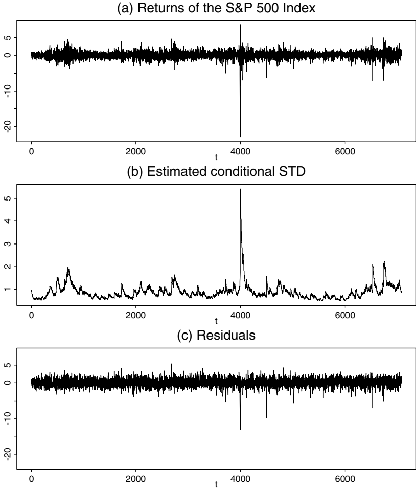
FIGURE 4.18. Time plots of (a) the S&P 500 returns \{X_t\} , (b) the estimated conditional standard deviations \{\hat{\sigma}_t\} given in (4.57), and (c) the residual \{\hat{\varepsilon}_t = X_t/\hat{\sigma}_t\} . The estimates were derived based on a GARCH(1, 1) model with t -distributed \varepsilon_t with the estimated degrees of freedom 7.41.
