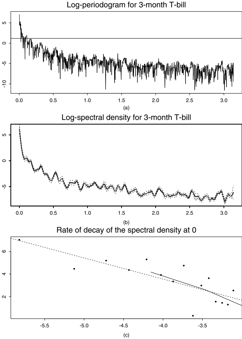
FIGURE 7.5. (a) Log-periodogram of \{Y_k - C_0\} against its Fourier frequency \{\omega_k\} . The bar indicates a 95% confidence upper limit above \log(\frac{\sigma^2}{2\pi}) . (b) Estimated log-spectral density by the local likelihood method \hat{m}_{LK} (solid curve) and the least-squares method \hat{m}_{LS} (thick dashed-curve) along with the 95% point-wise confidence intervals (7.26) (long dashed-curve). (c) The scatterplot of the log-periodogram of \{Y_k - C_0\} against \{\log(\omega_k)\} at low frequencies \omega_k \leq 30\pi/2112 along with the least-squares fit (dashed line). The solid curve is the plot of the estimated log-spectral density against its log-frequency.
