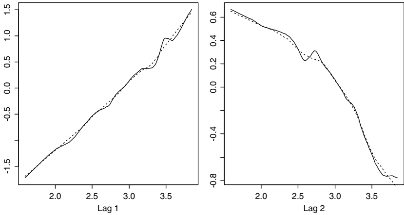
FIGURE 9.6. Estimated functions \hat{f}_1(\cdot) (left-panel) and \hat{f}_2(\cdot) (right-panel) for the Canadian lynx data using the backfitting algorithm with bandwidth selected by (8.51) (solid curves) and by the user (dashed curves).
