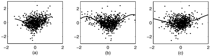
FIGURE 8.15. The observed series y_t is plotted against (a) index \beta_1^T \mathbf{X}_t ; (b) index \beta_2^T \mathbf{X}_t ; and (c) index \beta_3^T \mathbf{X}_t . The lines are drawn simply by polynomial regression to make the trends more visualizable. Adapted from Xia, Tong, Li, and Zhu (2002) with permission from the Royal Statistical Society.
