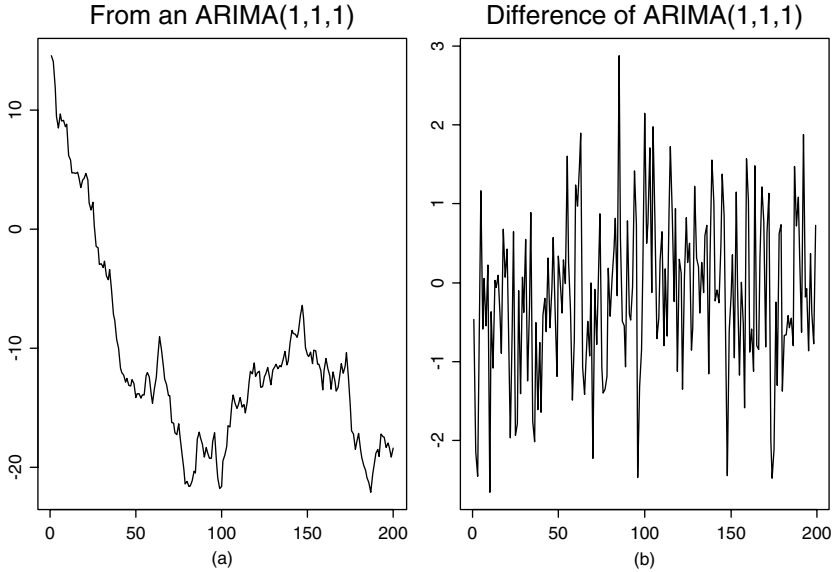
FIGURE 1.8. (a) A realization of a time series from ARIMA(1, 1, 1) given by (1.4). The series exhibits an obvious time trend. (b) The first-order difference of the series.
