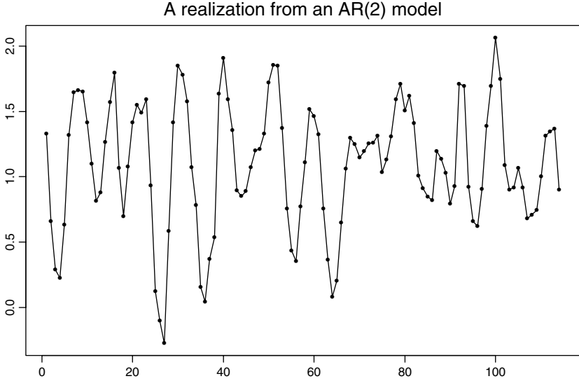
FIGURE 1.7. A length of 114 time series from the AR(2) model X_t = 1.07 + 1.35X_{t-1} - 0.72X_{t-2} + \varepsilon_t with \{\varepsilon_t\} \sim_{\text{i.i.d.}} N(0, 0.24^2) . The parameters are taken from the AR(2) fit to the lynx data.
