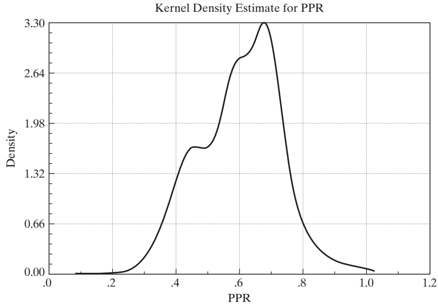
FIGURE 16.1 Probit Probabilities.
