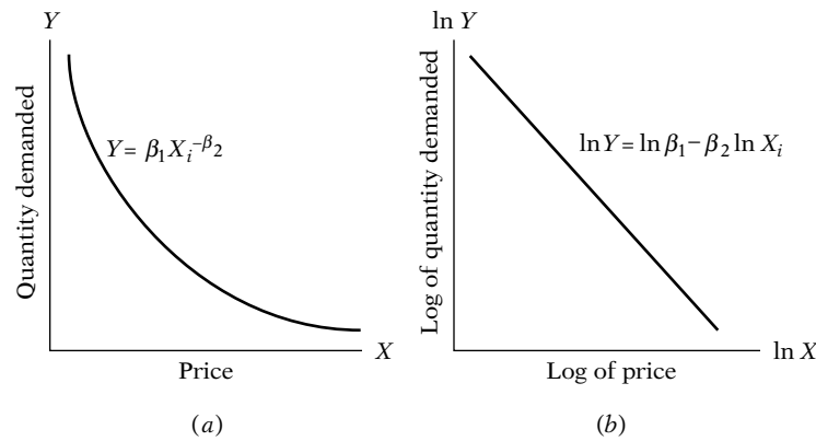
FIGURE 6.3 Constant-elasticity model.
