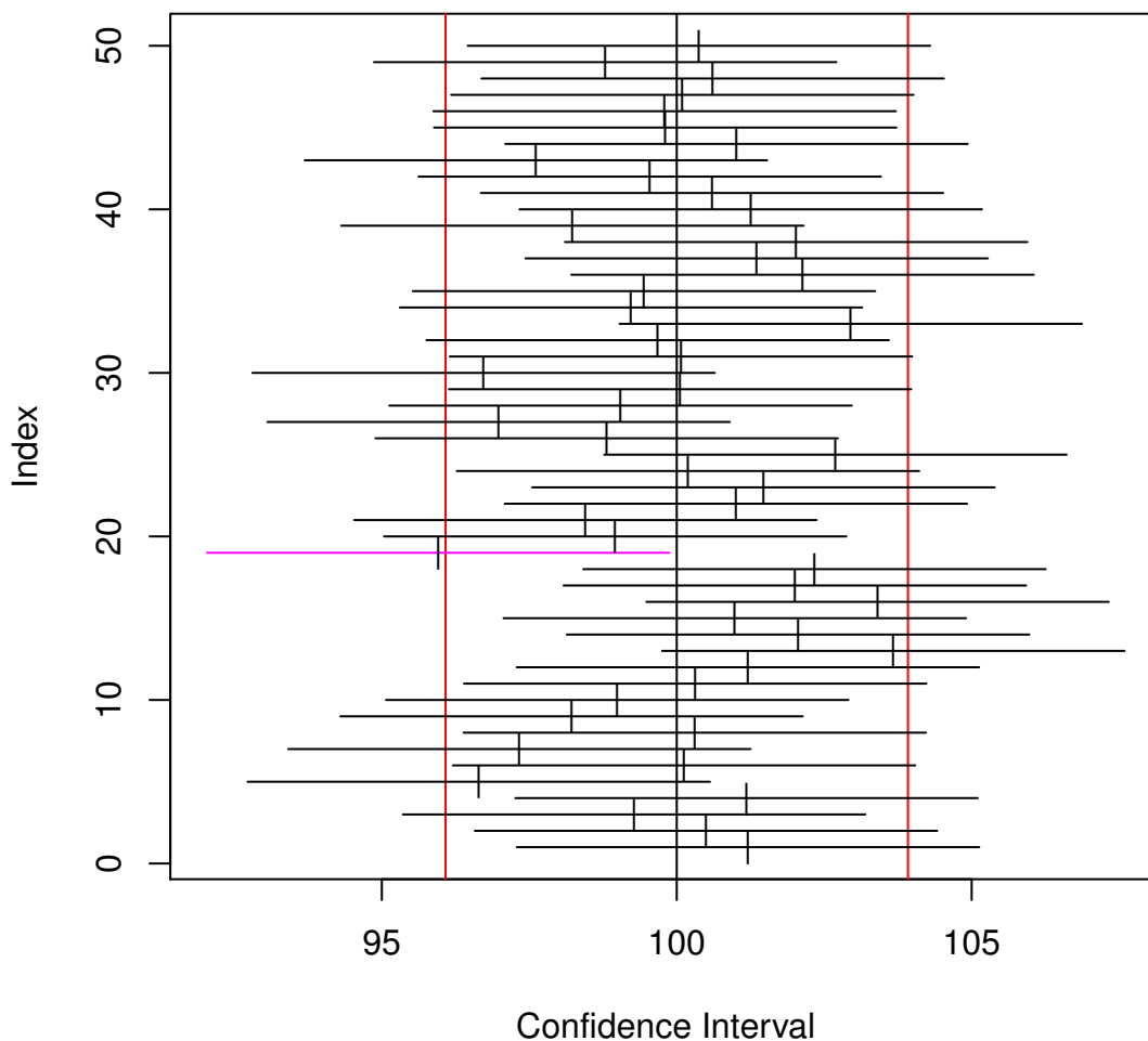
Figure 9.2.1: Simulated confidence intervals
