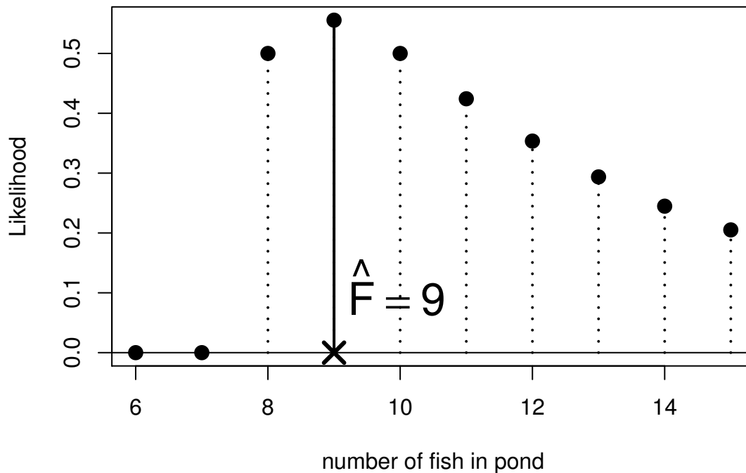
Figure 9.1.1: Capture-recapture experiment
