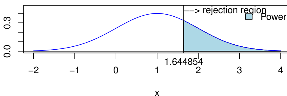
Figure 10.7.1: Plot of significance level and power
