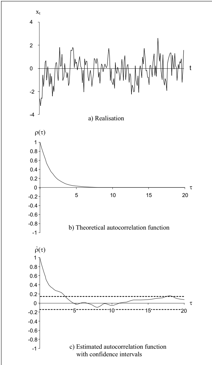
Figure 2.2: AR(1) process with \alpha = 0.5
