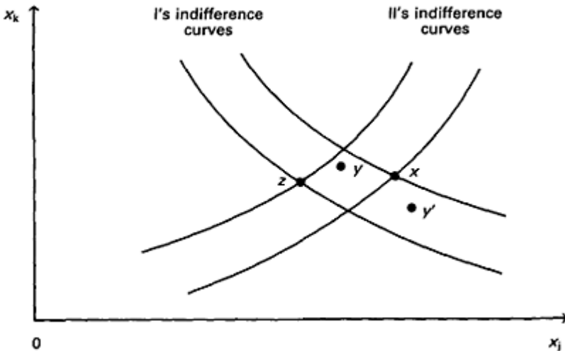
Figure 8.2 Extremal restrictedness
