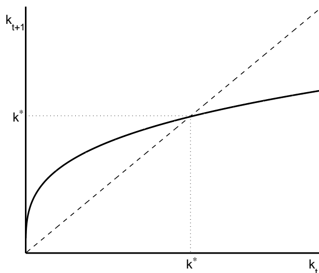
Figure 8.1: Global dynamics
