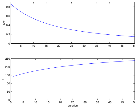
Figure 21.2.1: Top panel: replacement ratio c/w as a function of duration of unemployment in Shavell-Weiss model. Bottom panel: effort a as function of duration.
