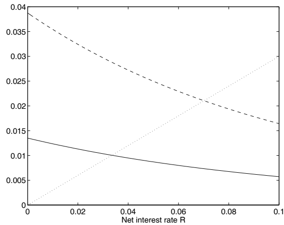
Figure 14.6.1: Interest rates in a version of Romer’s (1987) model of research and monopolistic competition. The dotted line is the linear relationship \kappa R , while the solid and dashed curves depict \Omega_m(R) and \Omega_s(R) , respectively. The intersection between \kappa R and \Omega_m(R) [ \Omega_s(R) ] determines the interest rate along a balanced growth path for the laissez-faire economy (planner allocation), as long as R \geq \beta^{-1} - 1 . The parameterization is \alpha = 0.9 , \kappa = 0.3 , and L = 1 .
