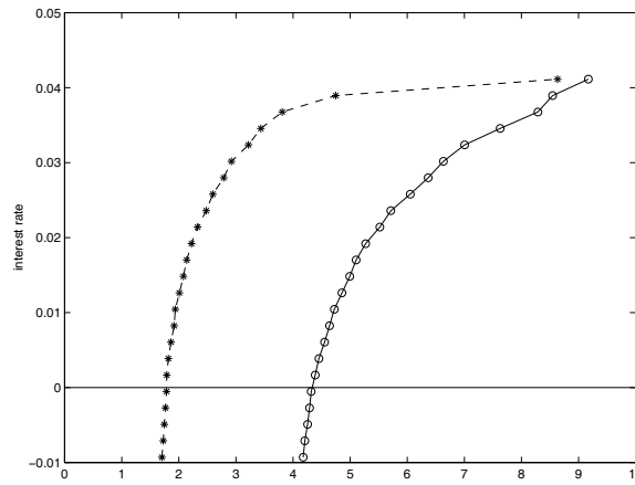
Figure 17.7.1: Two Ea(r) curves when b = 0 and the endowment shock s is i.i.d. but with different variances; the curve with circles belongs to the economy with the higher variance.
