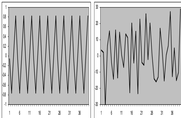
Figure 2.3: For 0 \leq \omega_1 < \dots < \omega_N \leq \pi , q_t = \sum_{j=1}^N q_{jt} , where q_{jt} = \cos(\omega_j t)[a_j \cos(\lambda_j)] - \sin(\omega_j t)[a_j \sin(\lambda_j)] . Left panel: N = 2 . Right panel: N = 1000
